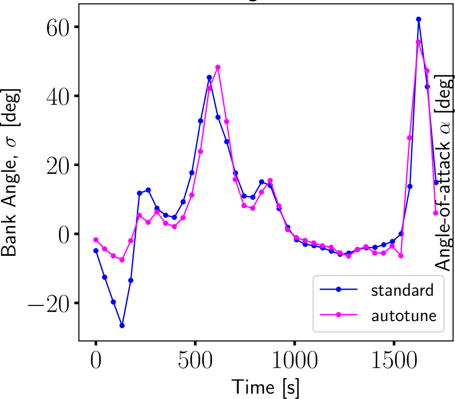
Bank Angle vs. Time
