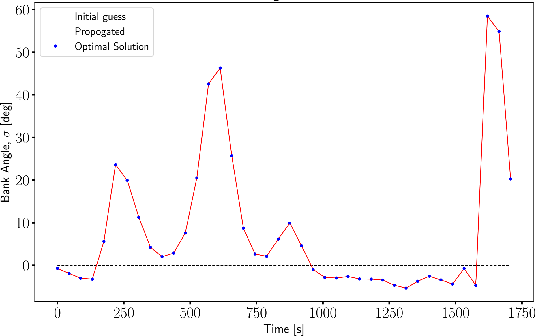
Bank Angle vs. Time
