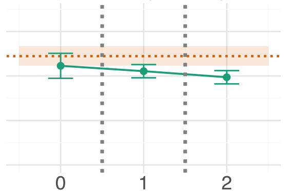
window typicality
