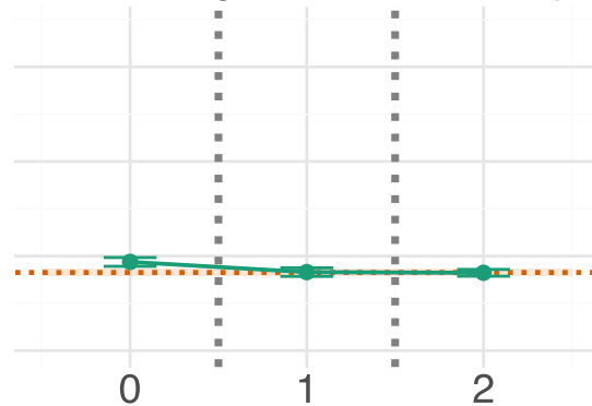
encoding compressibility
