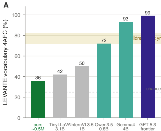
A: our model scored across all 159 items (real accuracy on the 100 in-vocabulary words, chance on the 59 it cannot attempt). Other models are prompted generatively — not a matched protocol. B: 76 items with a child difficulty estimate.
