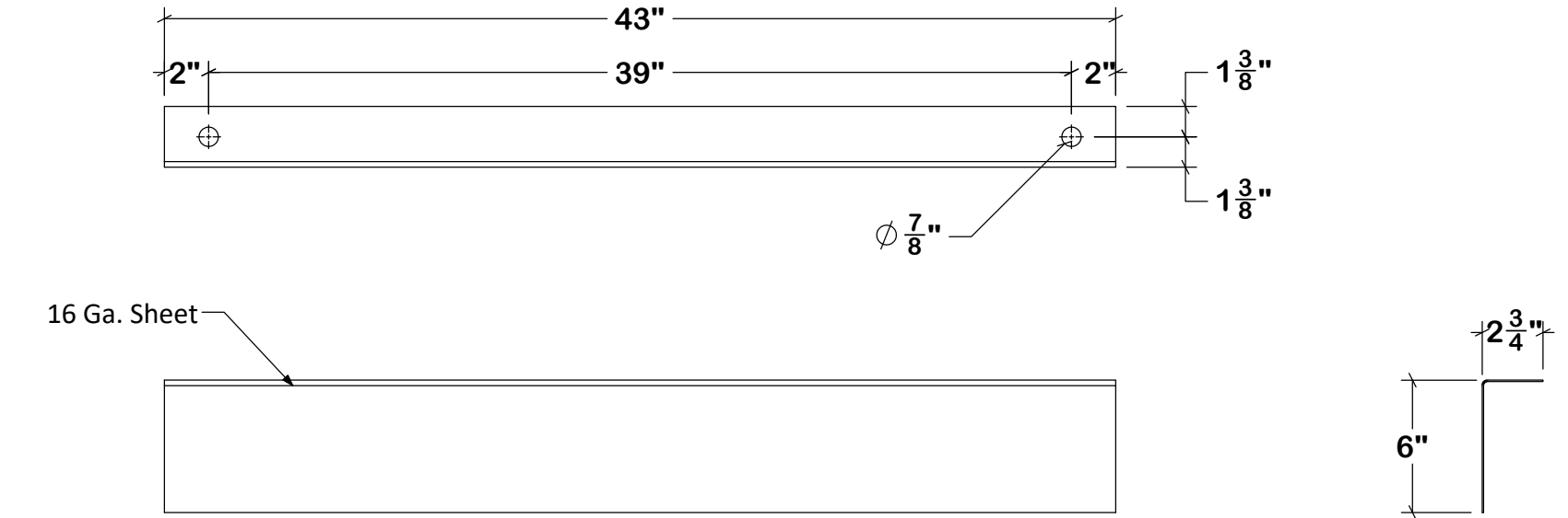
Large Riser Pan - QTY (34)
