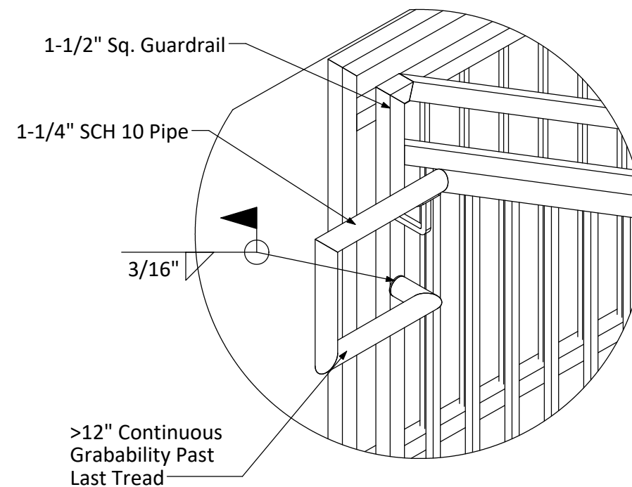
Top Handgrab Connection
