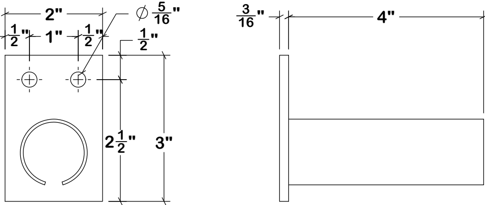
Pipe Sleeve Details
