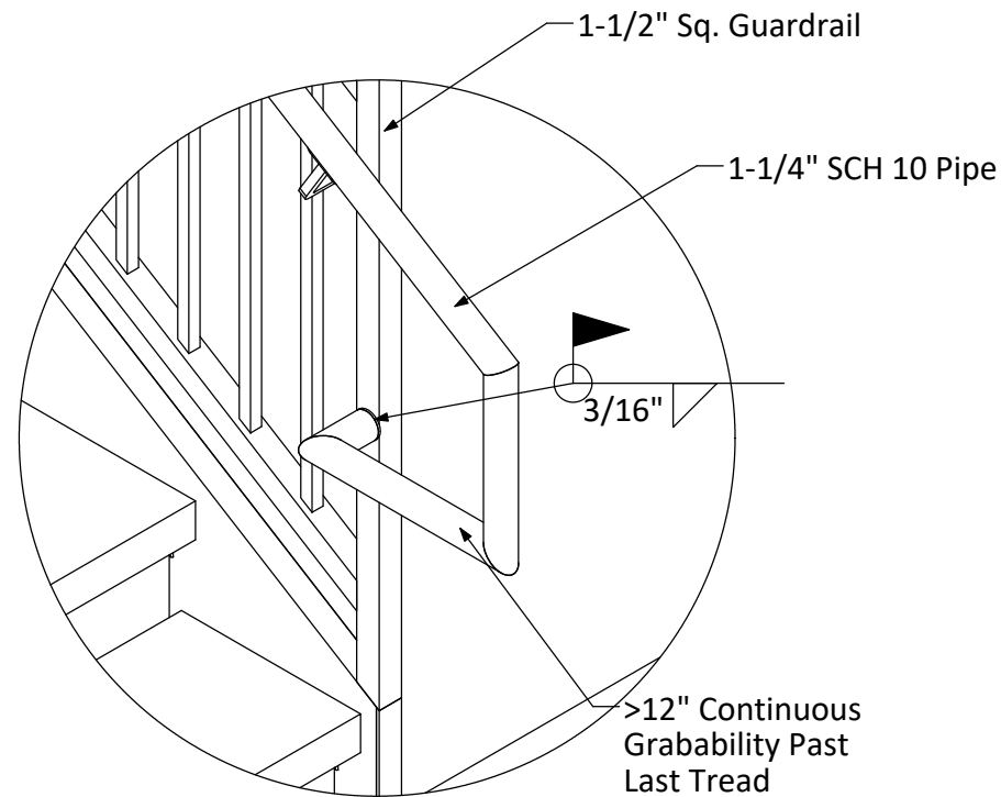
Bottom Handgrab Connection
