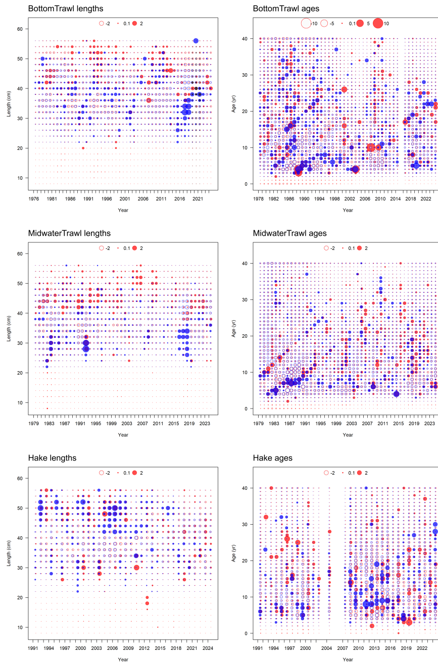
Figure 41: Pearson residuals for fits to length frequency data (left) and age frequency data (right) for landings from the trawl commercial fleets (rows). Filled circles indicate that the fitted proportion was less than the observed proportion. Red indicates females, blue males, and gray unsexed.
