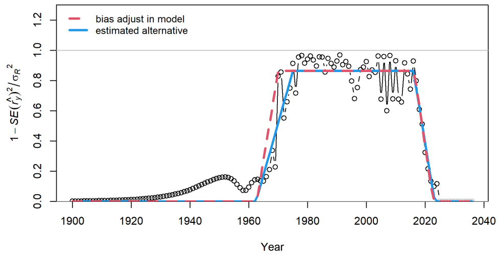
Figure 39: Estimated and input recruitment bias adjustment ramp. Red line shows current settings for bias adjustment ramp. Red line shows current settings for bias adjustment specified in the model. Blue line shows least squares estimate of alternative bias adjustment relationship for recruitment deviations.
