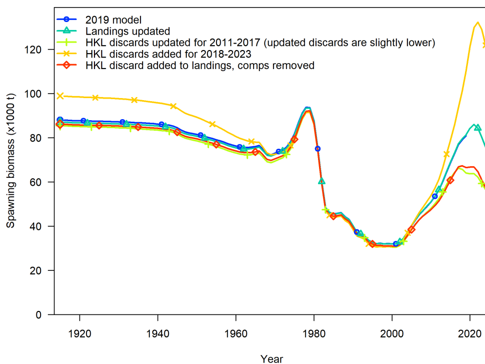
Figure 21: Spawning biomass with intermediate steps in hook-and-like discard data updates.
