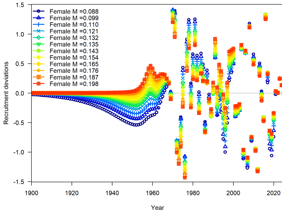
Figure 63: Time series of recruitment deviations for models with different fixed values of natural mortality ( M ). The base model has M = 0.135 .
