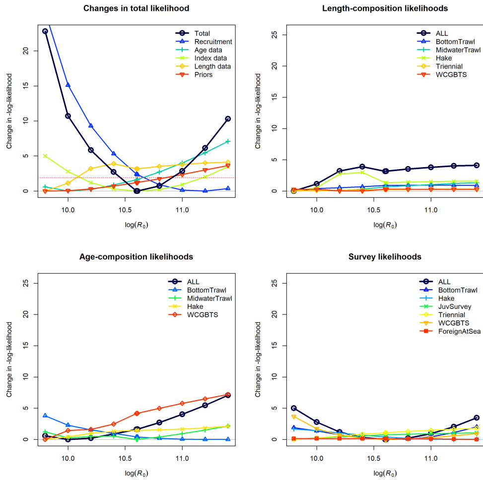
Figure 59: Likelihood components in the likelihood profile for unfished equilibrium recruitment ( R_0 )
