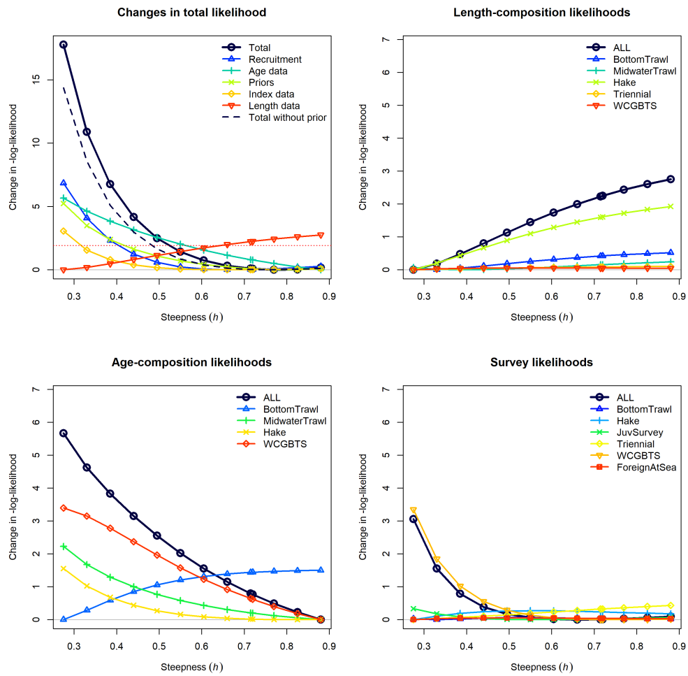
Figure 60: Likelihood components in the likelihood profile for steepness ( h ).
