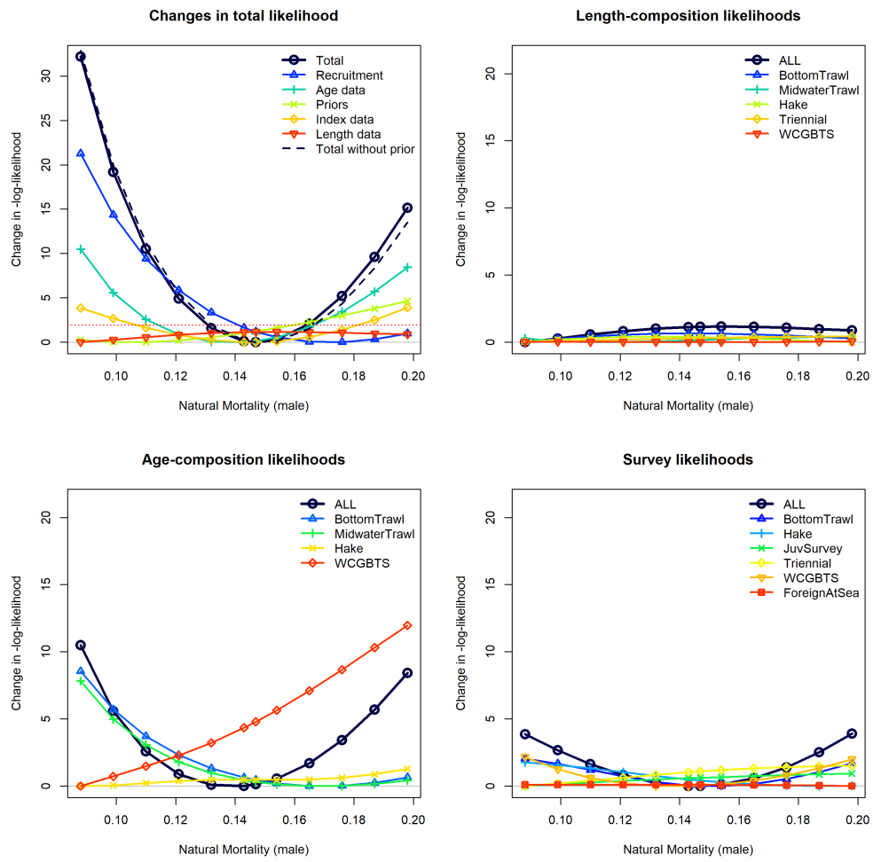
Figure 62: Likelihood components in the likelihood profile for male natural mortality ( M ). Female natural mortality is set to the same value.
