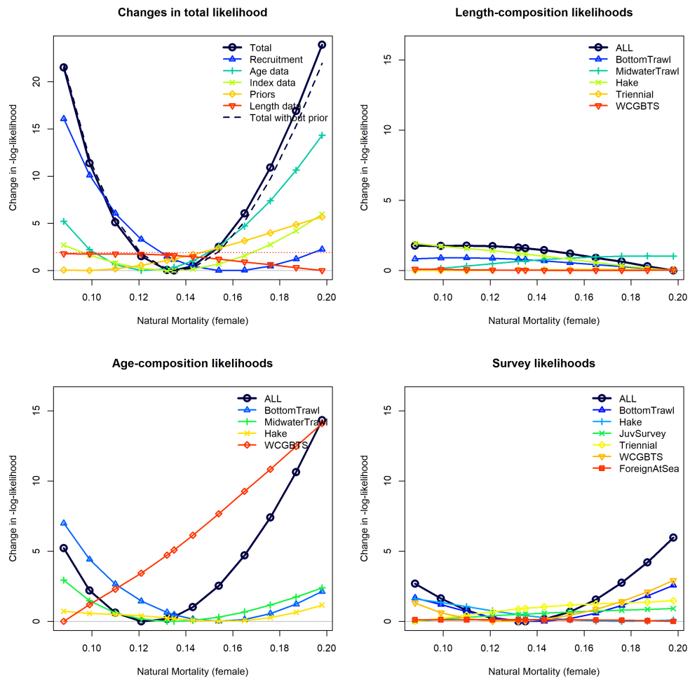
Figure 61: Likelihood components in the likelihood profile for female natural mortality ( M ). Male natural mortality are set to the same value.
