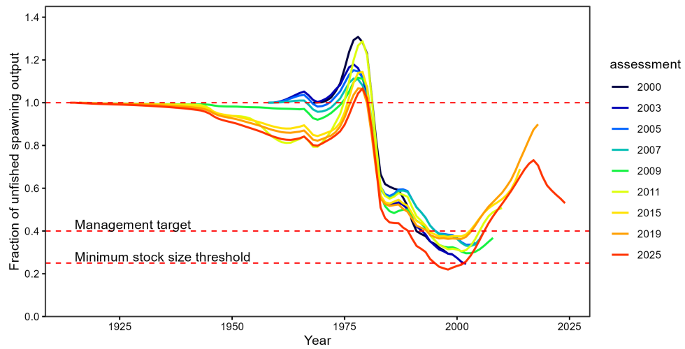
Figure 58: Estimated fraction of unfished spawning output from past assessments in comparison with the current assessment. The units of spawning output differ among assessments but the ratio remains comparable.
