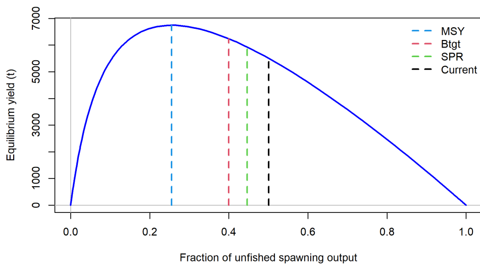
Figure 64: Estimated plot of equilibrium yield vs the fraction of unfished biomass.
