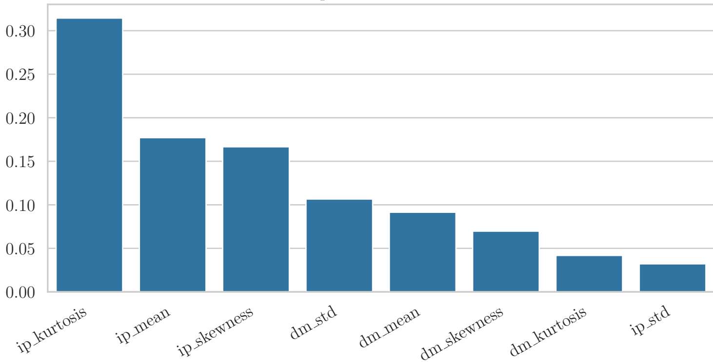
Feature Importances – random_forest
