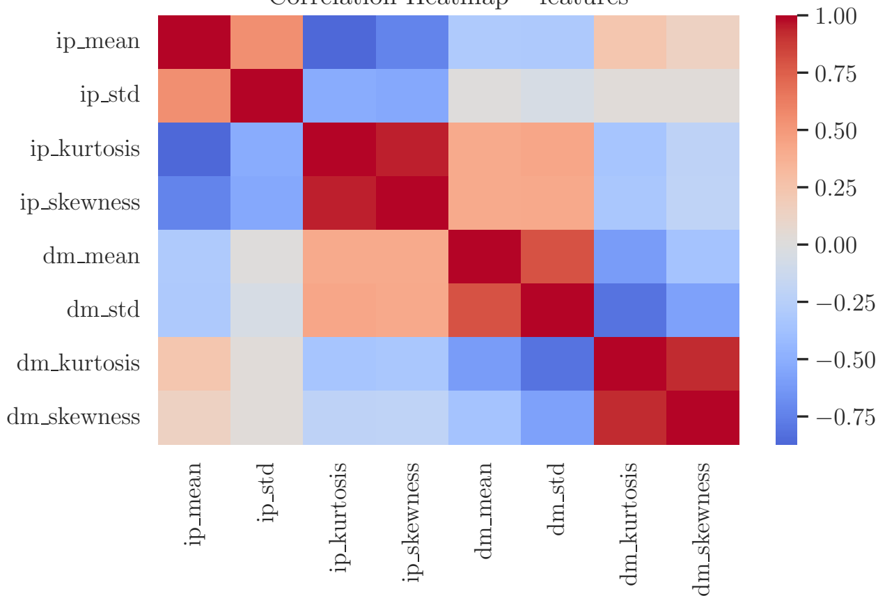
Correlation Heatmap – features
