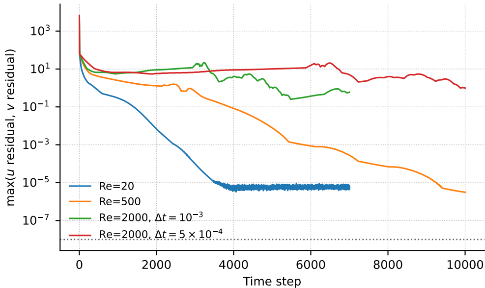
QUICK residual histories
