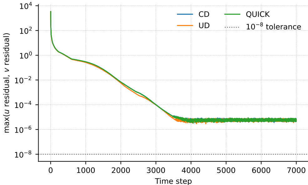
Residual histories at Re=20
