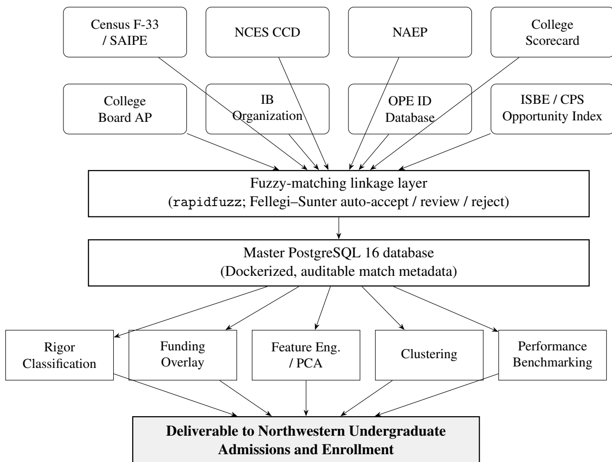
Figure 2: Data architecture: eight public sources are linked through a fuzzy-matching layer implementing a Fellegi–Sunter accept/review/reject decision rule (Section 2.5) into a single Dockerized master database, which feeds the five analytical components described in Section 4.
