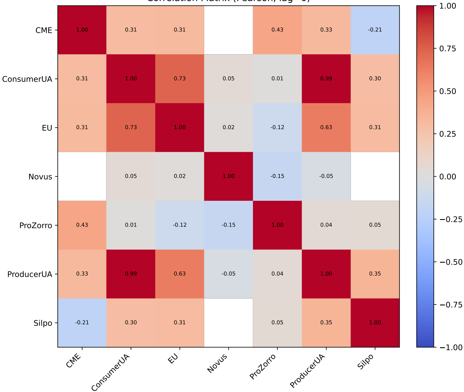
Correlation Matrix (Pearson, lag=0)
