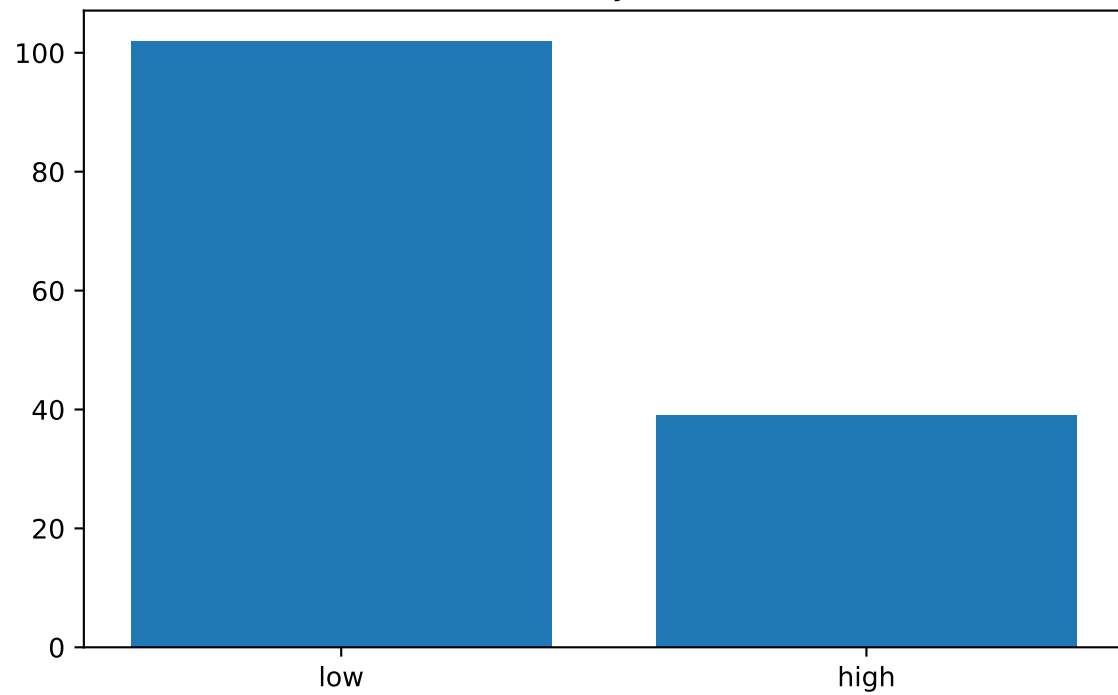
Stability Risk
