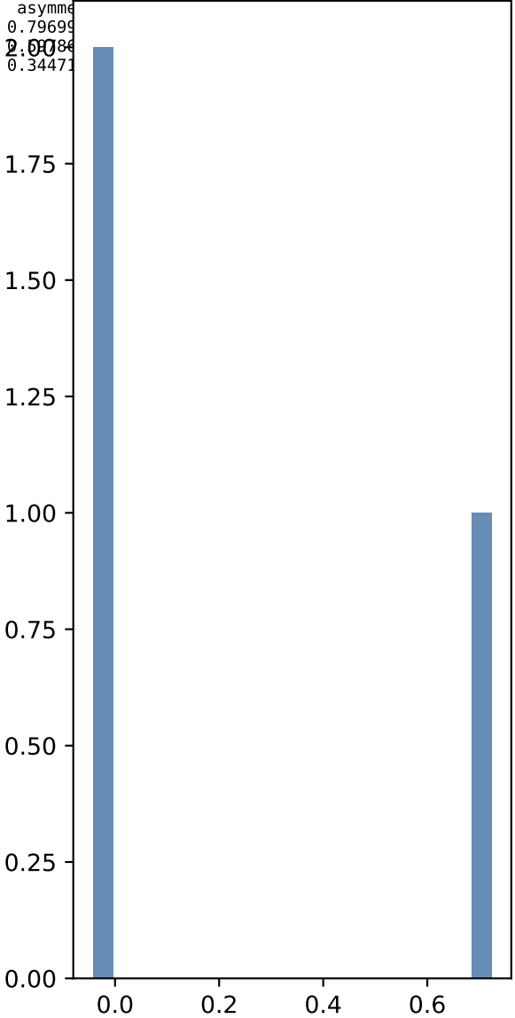
Distribution: short_run_coef
