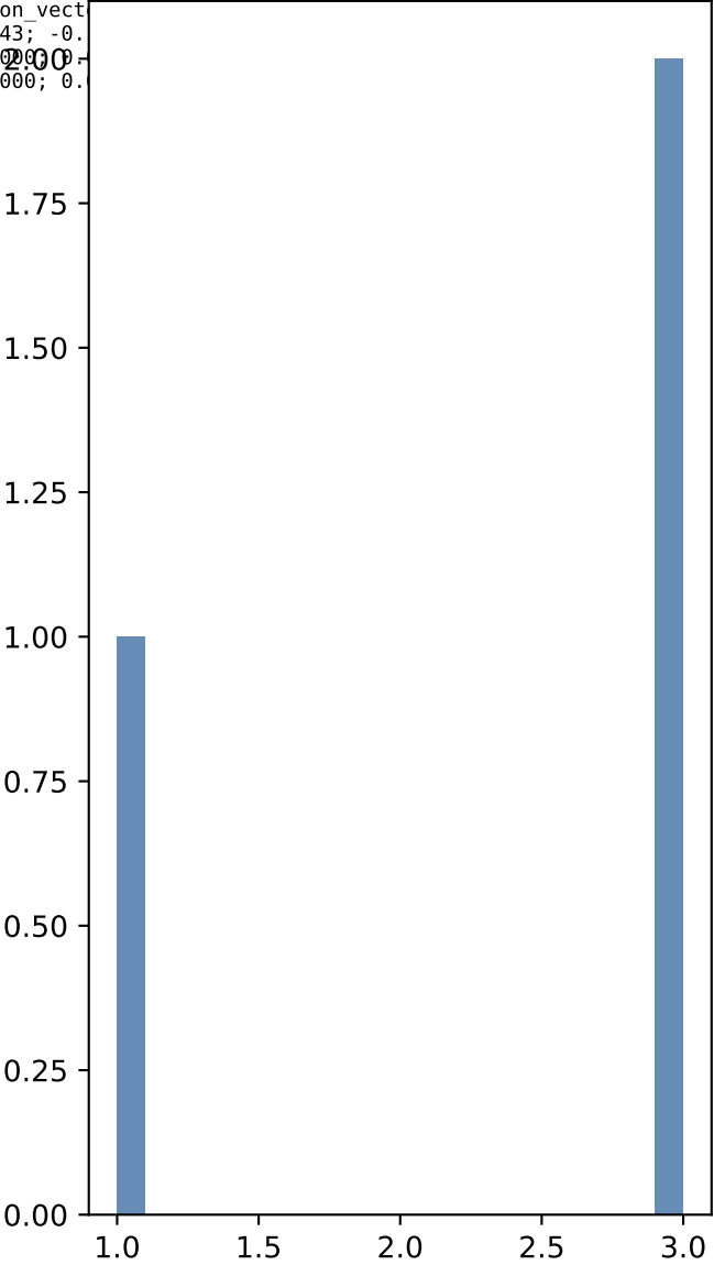
Distribution: cointegration_rank
