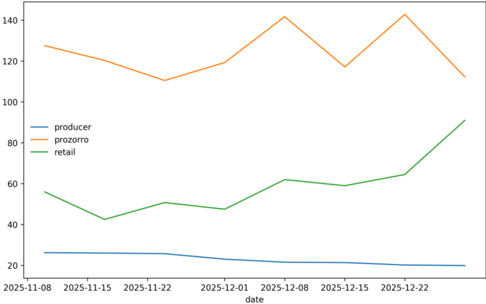
time_series_promo_controlled.png sour_cream | novus | promo_controlled
