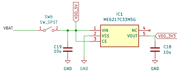
5V (USB OR BATTERY) TO 3.3V LDO
