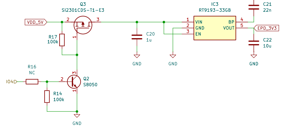
5V TO DEDICATED 3.3V FOR E-PAPER
