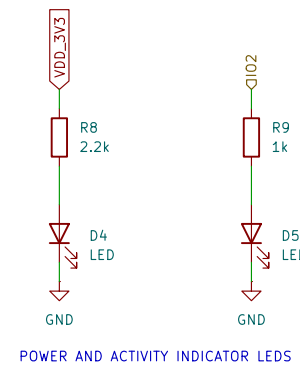
POWER AND ACTIVITY INDICATOR LEDS
