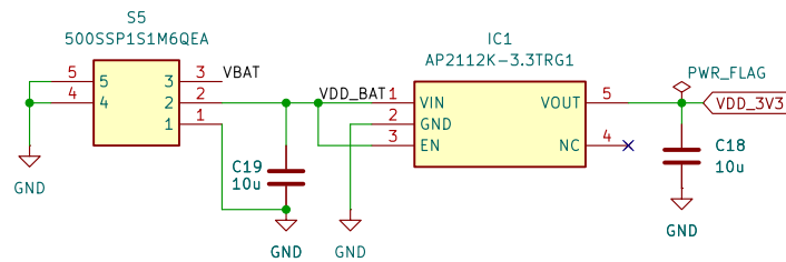
5V (USB OR BATTERY) TO 3.3V LDO
