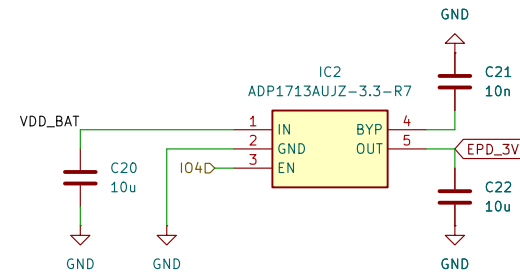
5V TO DEDICATED 3.3V FOR E-PAPER
