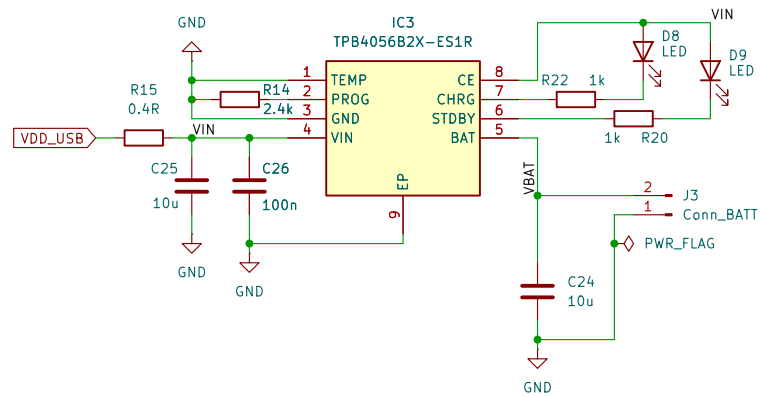
BATTERY CHARGING CIRCUIT VIA USB
