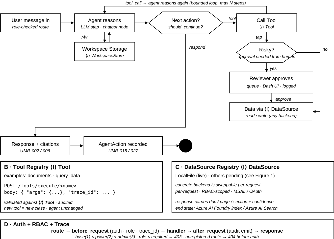
Figure 2 · Agent loop with HITL branch, Tool registry, DataSource registry, auth cluster.
