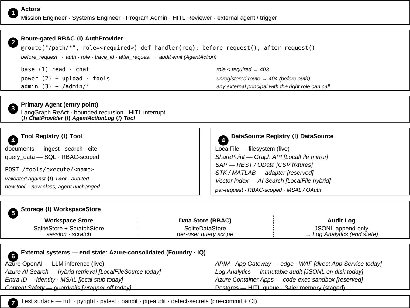
Figure 1 · L2 — Containers, Actors, External Systems
