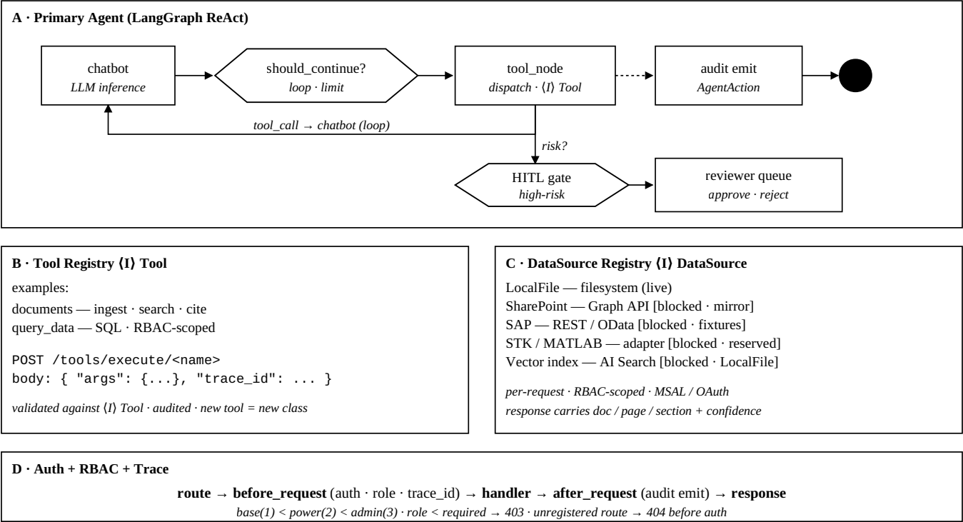
Figure 2 · Agent loop with HITL branch, Tool registry, DataSource registry, auth cluster.
