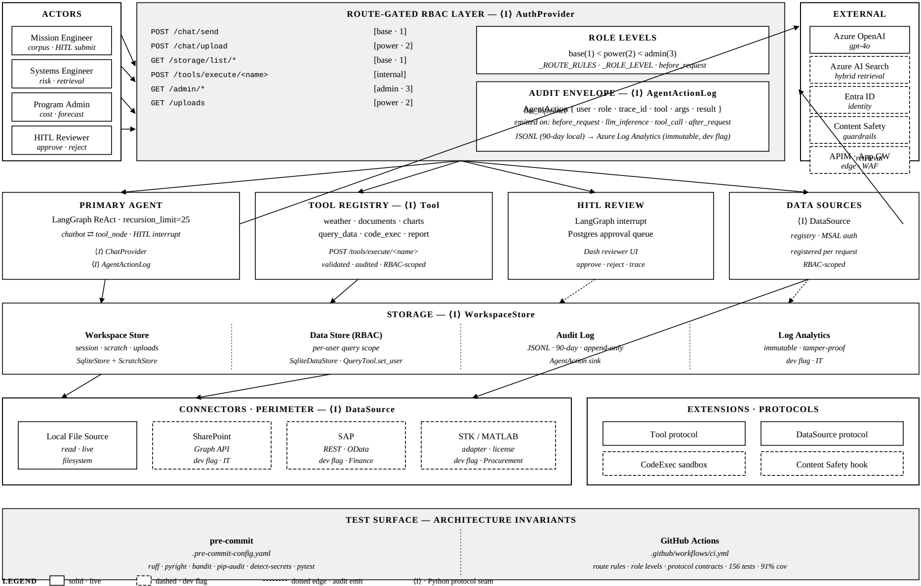
Figure 1 · Actors, external systems, routes, containers, and the audit + RBAC perimeters.
