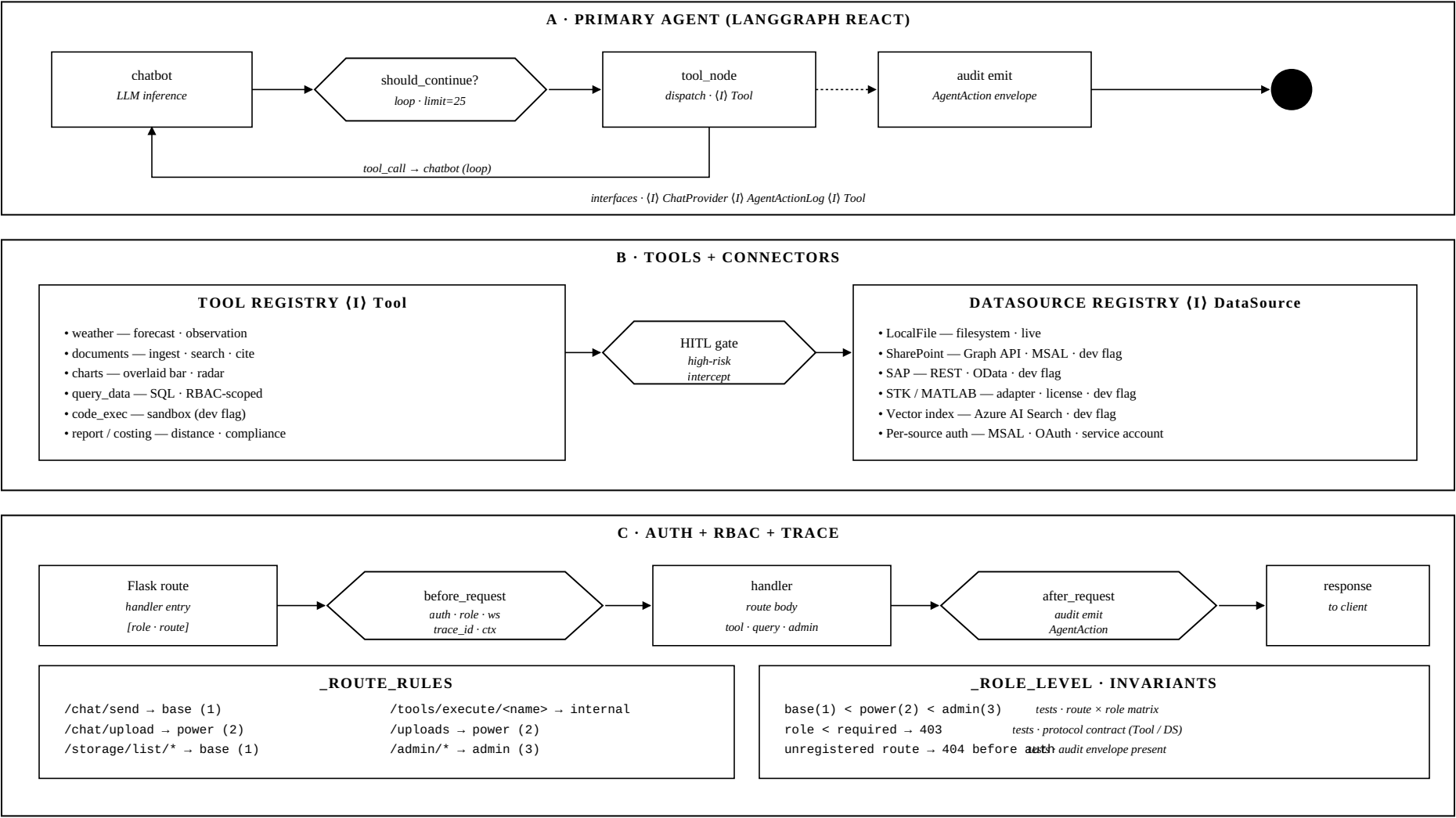
Figure 2 · Primary agent loop, tool/connector cluster, and auth cluster.
