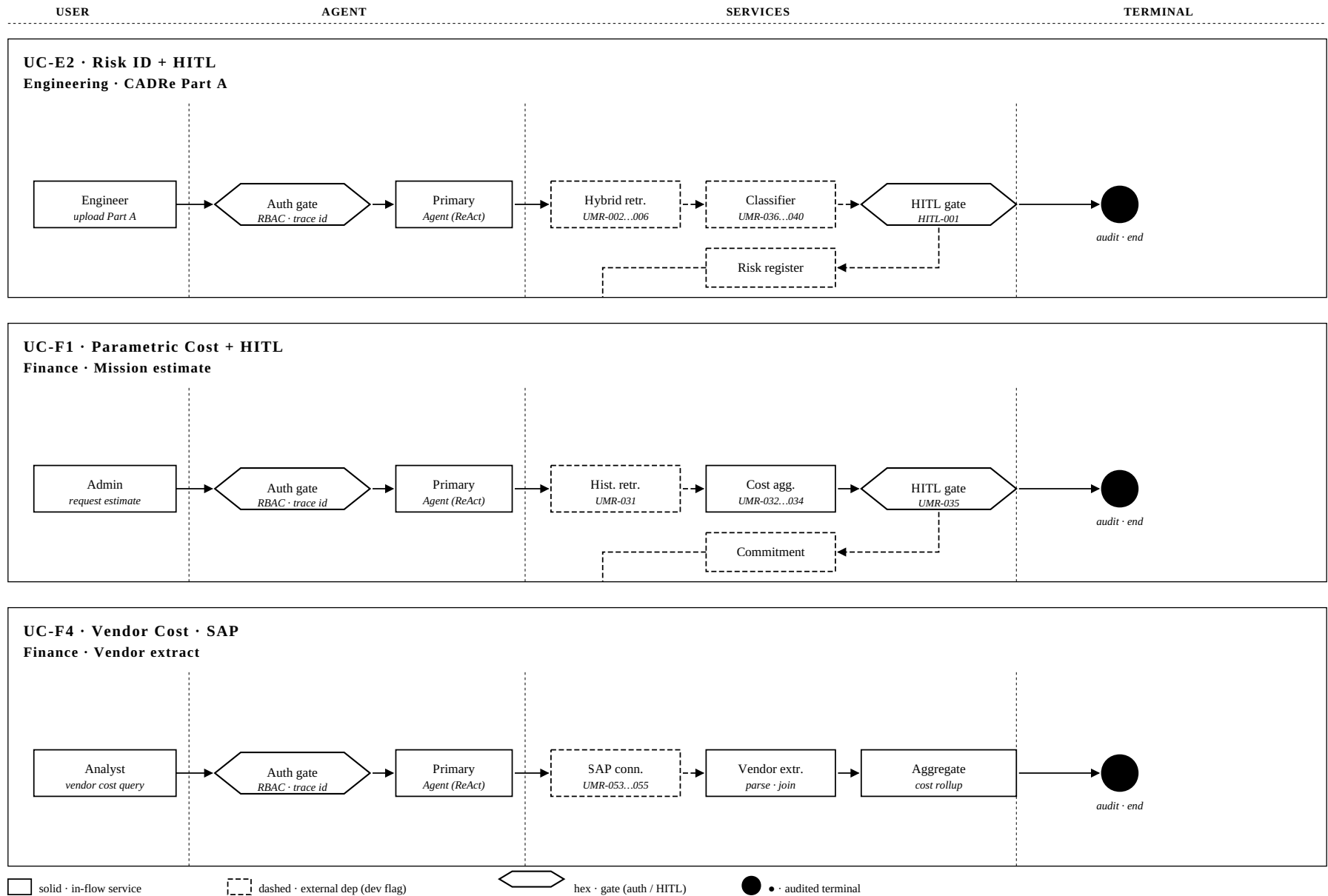
Figure 3 · Three use-case lanes laid out left-to-right with UC IDs and swim-lane dividers.
