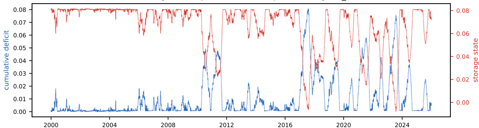
Cumulative deficit & storage state (peak deficit = required storage, S_{\text{tot}} =8.2% of annual)
