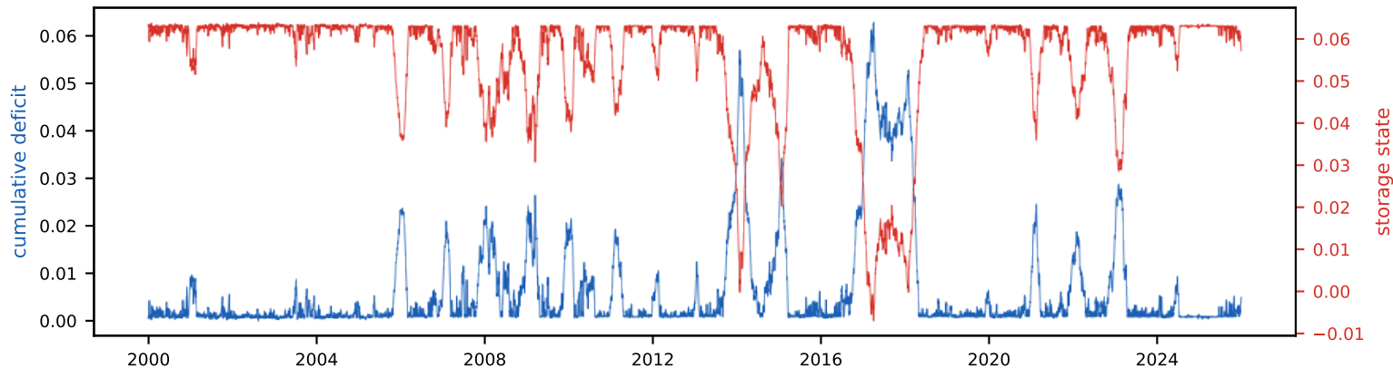
Cumulative deficit & storage state (peak deficit = required storage, S_{tot}=6.4\% of annual)
