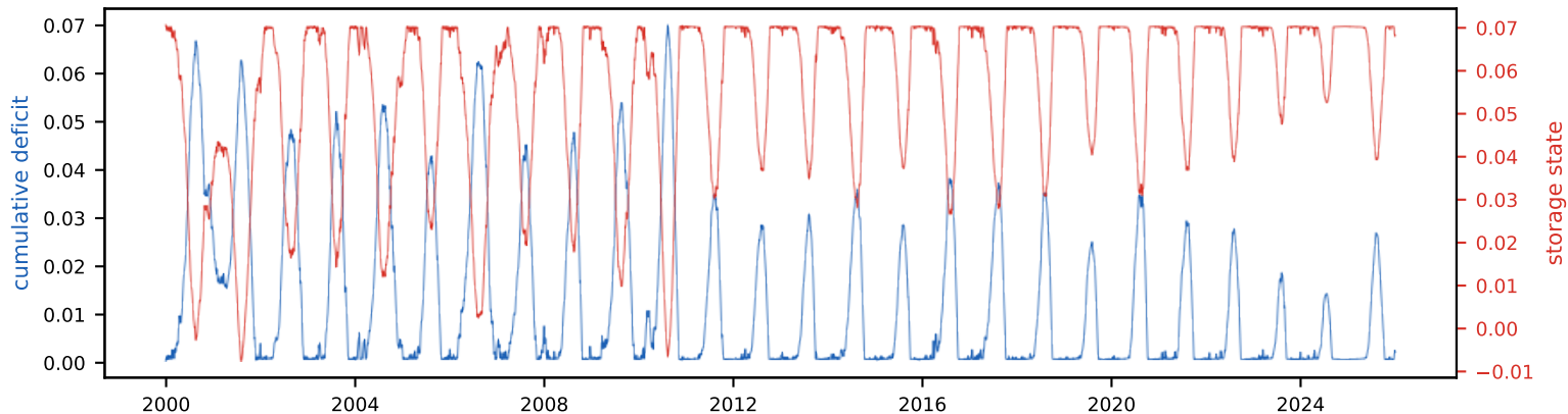
Cumulative deficit & storage state (peak deficit = required storage, S_{\text{tot}} =7.1% of annual)
