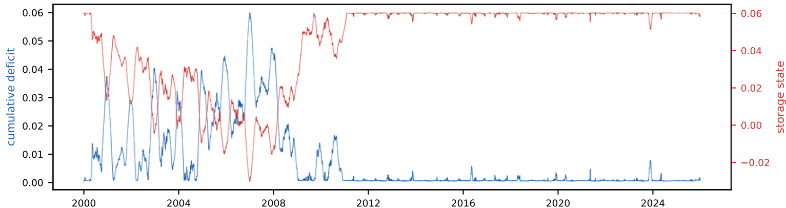
Cumulative deficit & storage state (peak deficit = required storage, S_{\text{tot}} =6.1% of annual)
