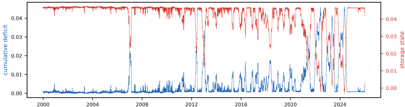
Cumulative deficit & storage state (peak deficit = required storage, S_{\text{tot}} =4.7% of annual)
