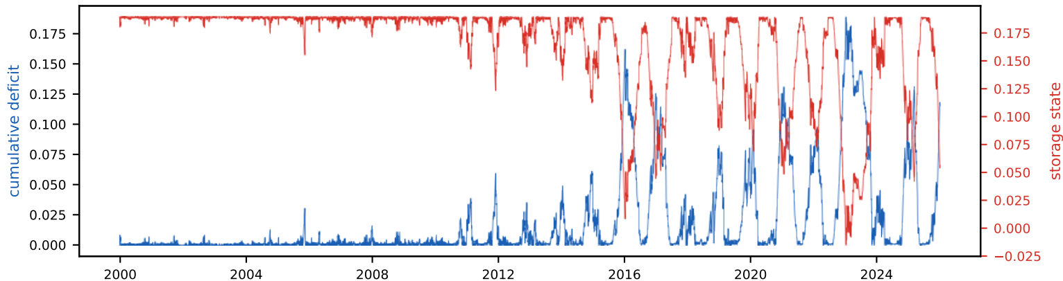
Cumulative deficit & storage state (peak deficit = required storage, S_{\text{tot}} =18.9% of annual)
