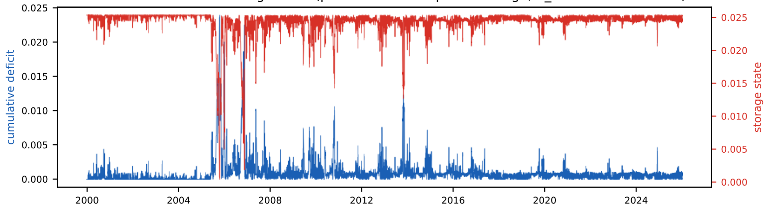
Cumulative deficit & storage state (peak deficit = required storage, S_{\text{tot}} =2.5% of annual)
