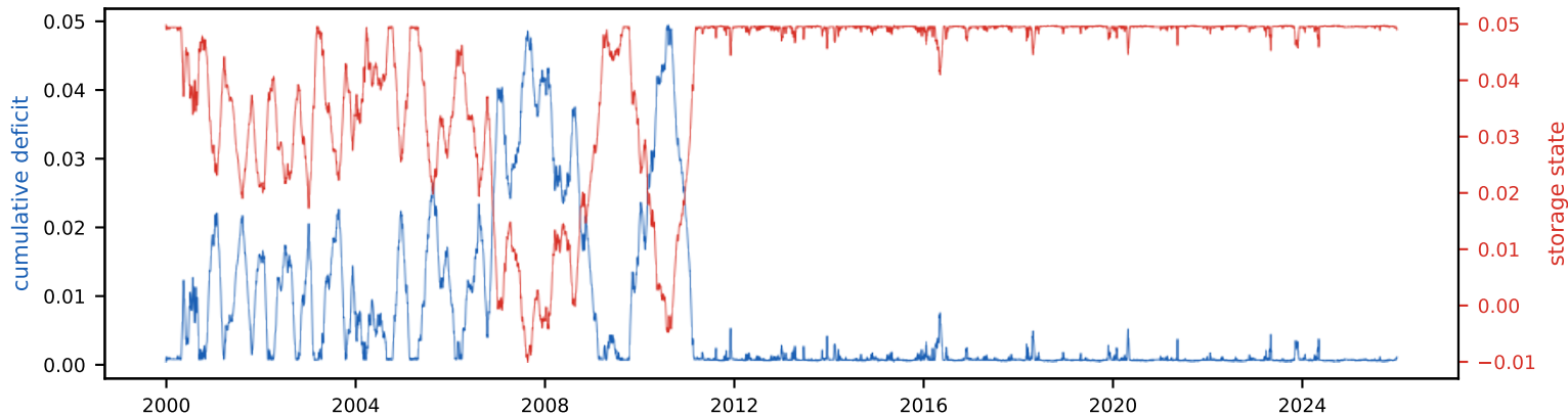
Cumulative deficit & storage state (peak deficit = required storage, S_{tot}=5.0\% of annual)
