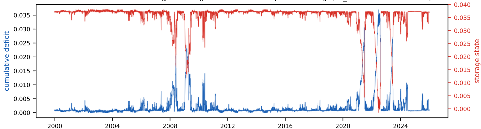
Cumulative deficit & storage state (peak deficit = required storage, S_{\text{tot}} =3.8% of annual)
