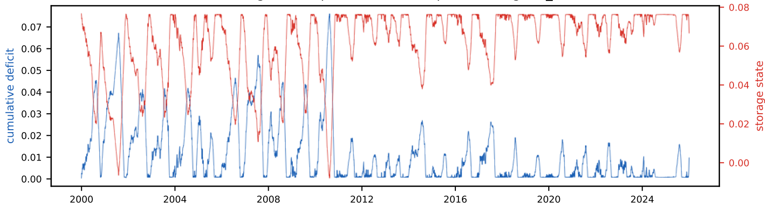
Cumulative deficit & storage state (peak deficit = required storage, S_{tot}=7.7\% of annual)
