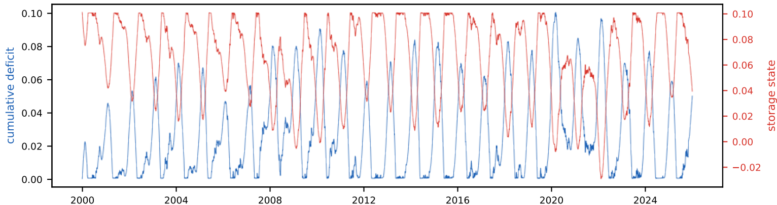
Cumulative deficit & storage state (peak deficit = required storage, S_{\text{tot}}=10.1\% of annual)
