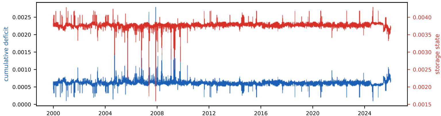
Cumulative deficit & storage state (peak deficit = required storage, S_{\text{tot}}=0.4\% of annual)
