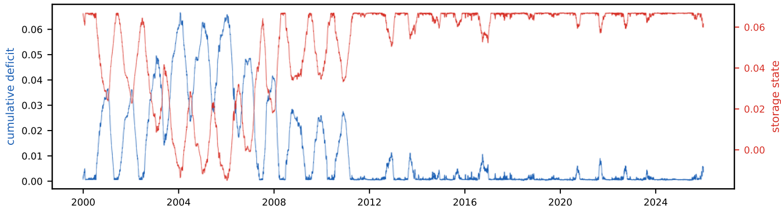
Cumulative deficit & storage state (peak deficit = required storage, S_{\text{tot}}=6.7\% of annual)
