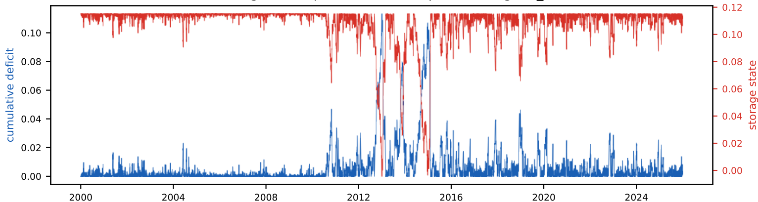
Cumulative deficit & storage state (peak deficit = required storage, S_{\text{tot}} =11.5% of annual)
