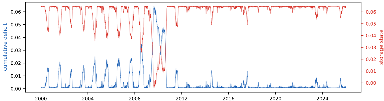
Cumulative deficit & storage state (peak deficit = required storage, S_{\text{tot}} =6.5% of annual)
