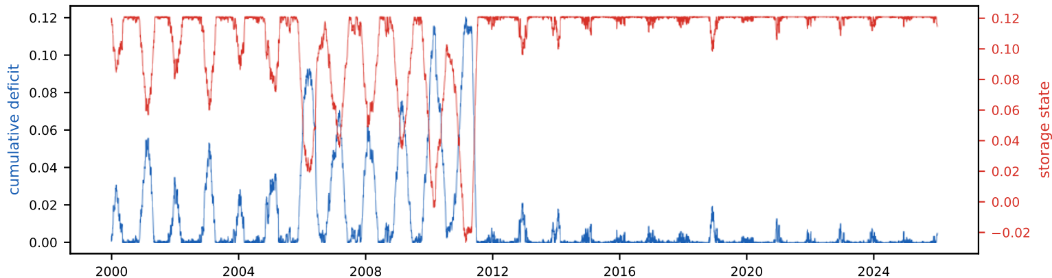
Cumulative deficit & storage state (peak deficit = required storage, S_{\text{tot}} =12.1% of annual)
