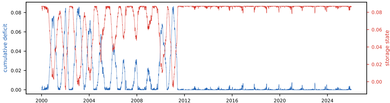
Cumulative deficit & storage state (peak deficit = required storage, S_{\text{tot}} =8.7% of annual)
