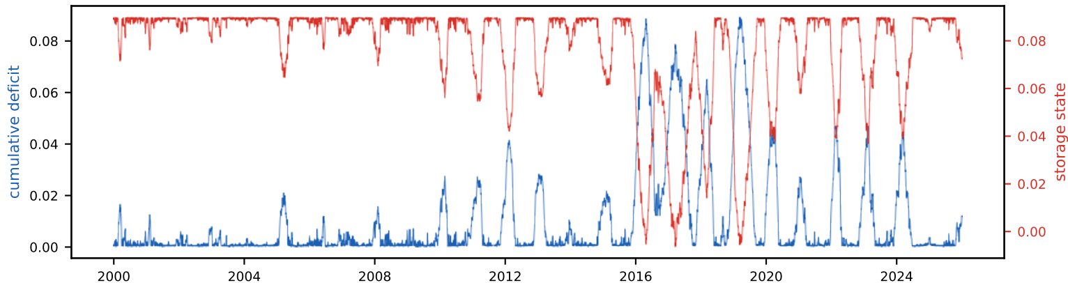
Cumulative deficit & storage state (peak deficit = required storage, S_{\text{tot}} =9.0% of annual)
