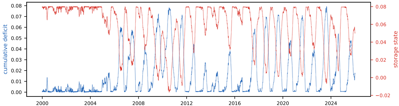
Cumulative deficit & storage state (peak deficit = required storage, S_{\text{tot}}=8.0\% of annual)
