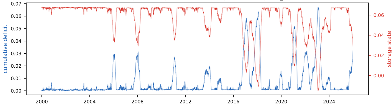
Cumulative deficit & storage state (peak deficit = required storage, S_{\text{tot}} =6.8% of annual)
