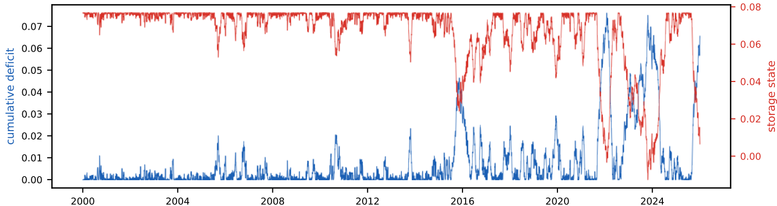
Cumulative deficit & storage state (peak deficit = required storage, S_{\text{tot}} =7.7% of annual)
