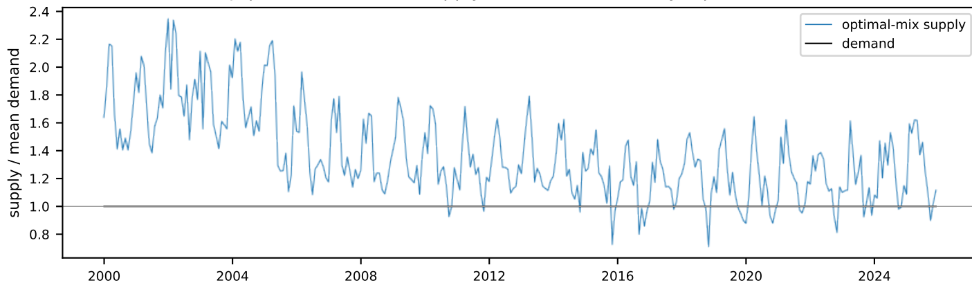
Japan — normalized supply vs demand (monthly, optimal mix)
