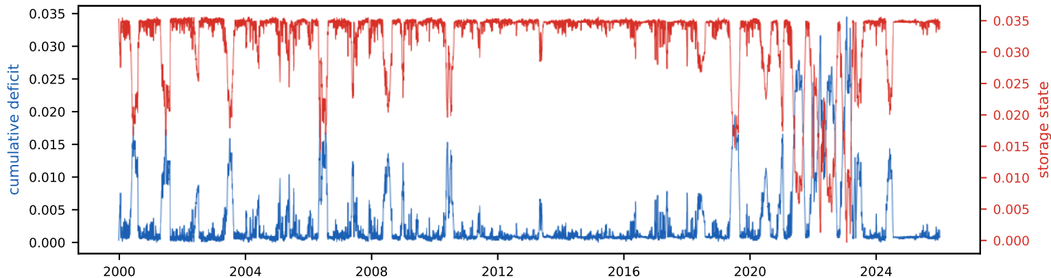
Cumulative deficit & storage state (peak deficit = required storage, S_{\text{tot}} =3.6% of annual)
