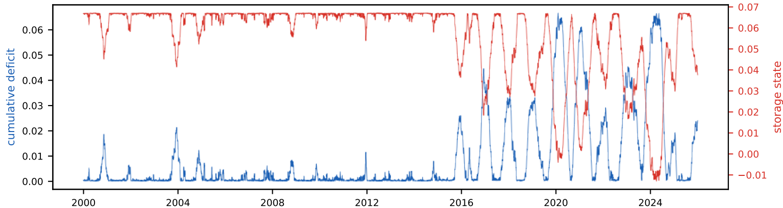
Cumulative deficit & storage state (peak deficit = required storage, S_{\text{tot}}=6.7\% of annual)
