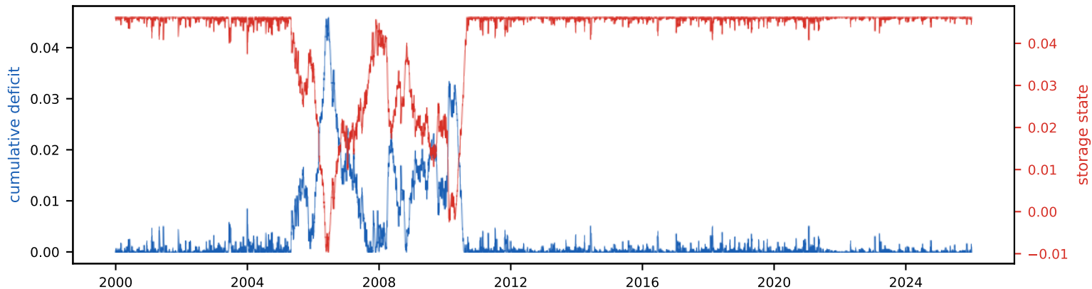
Cumulative deficit & storage state (peak deficit = required storage, S_{\text{tot}}=4.6\% of annual)
