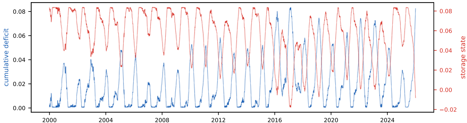
Cumulative deficit & storage state (peak deficit = required storage, S_{\text{tot}} =8.4% of annual)
