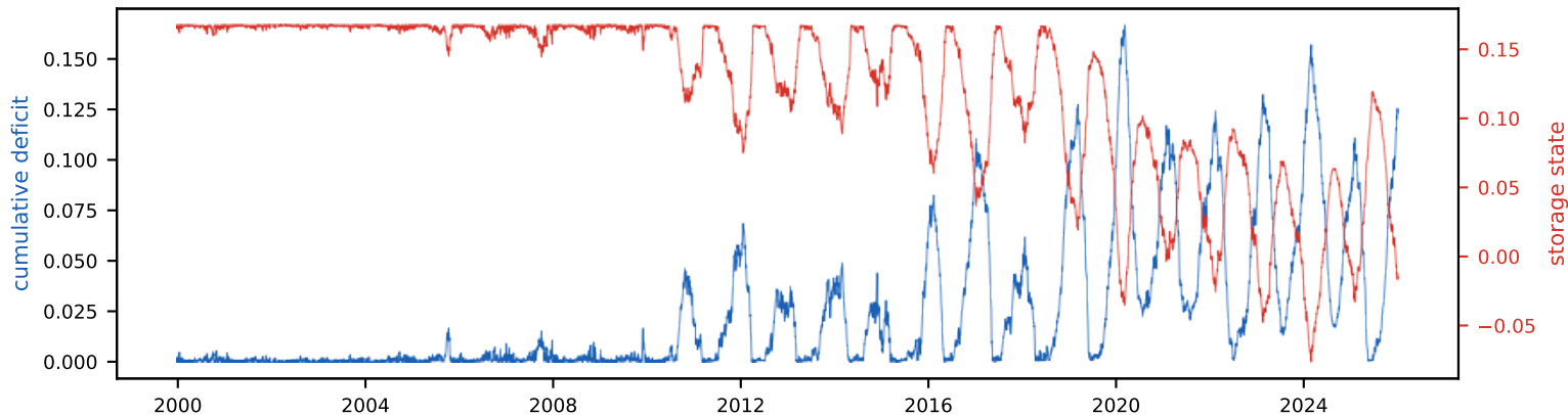
Cumulative deficit & storage state (peak deficit = required storage, S_{tot} =16.7% of annual)
