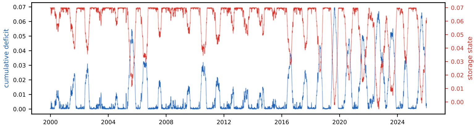
Cumulative deficit & storage state (peak deficit = required storage, S_{\text{tot}} =7.0% of annual)
