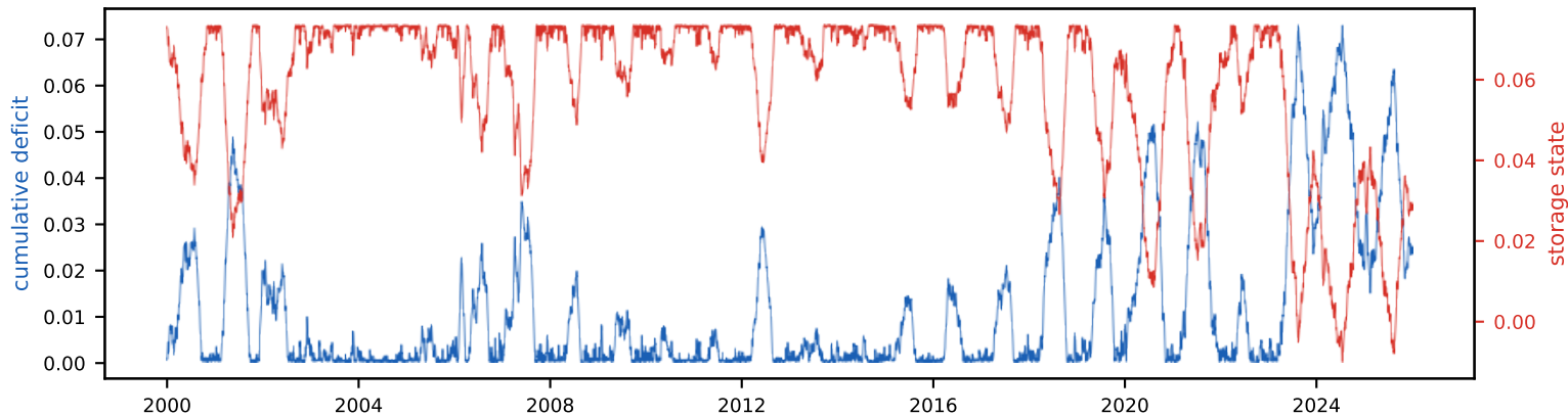
Cumulative deficit & storage state (peak deficit = required storage, S_{\text{tot}} =7.4% of annual)
