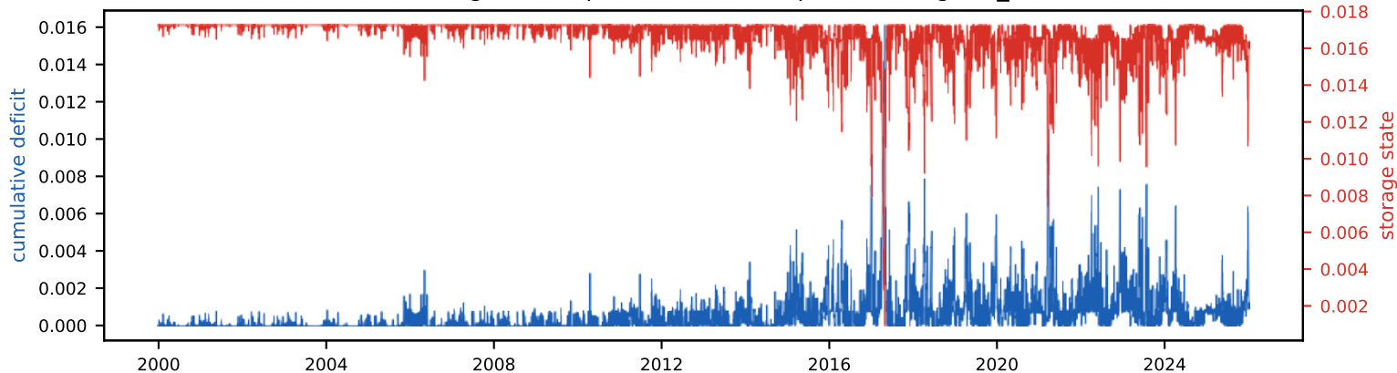
Cumulative deficit & storage state (peak deficit = required storage, S_{\text{tot}} =1.7% of annual)
